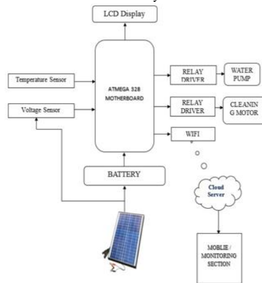
Block Diagram of IoT Based Solar Power Monitoring & Control System
