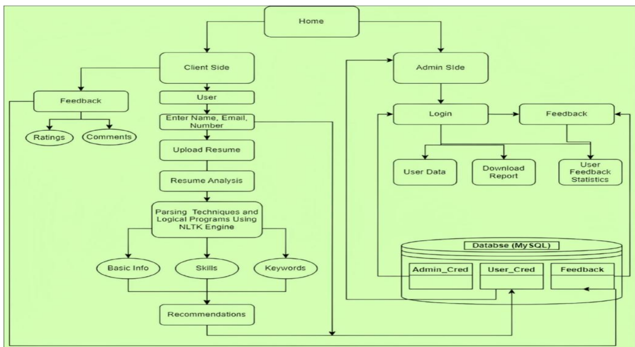
Figure 1 | Flow graph.
