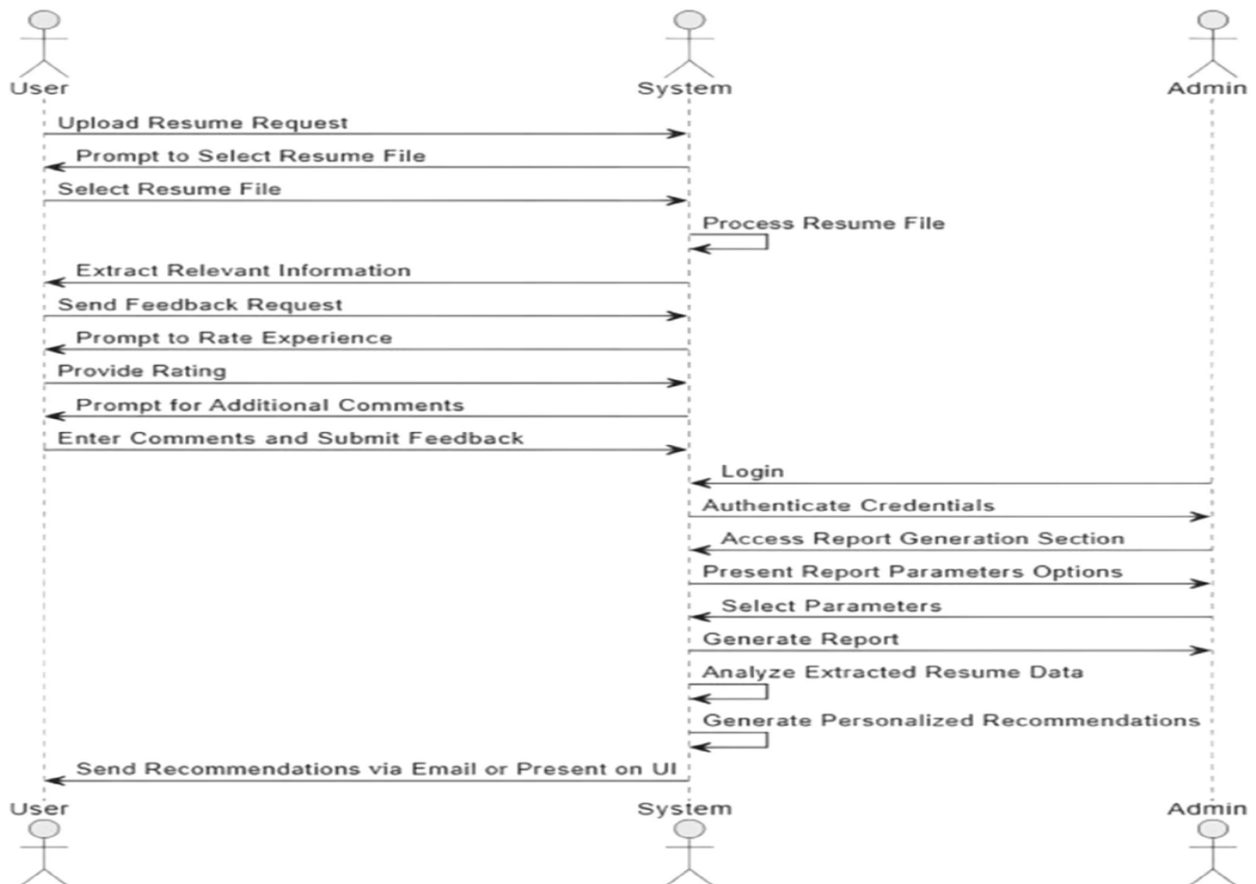
Figure 9 | Sequence diagram of resume analyzer.
