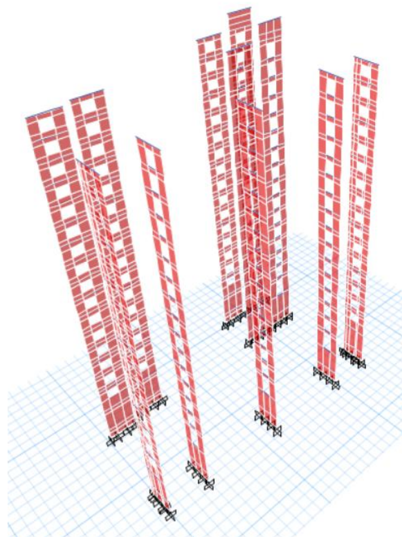
Figure 2: Etabs 3-D View for Vertical Opening (Model-1)
