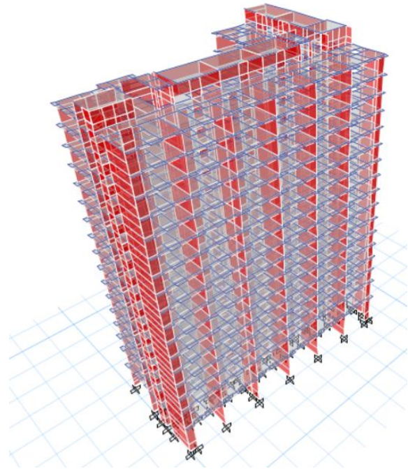
Figure 1: Etabs 3-D View for Building
