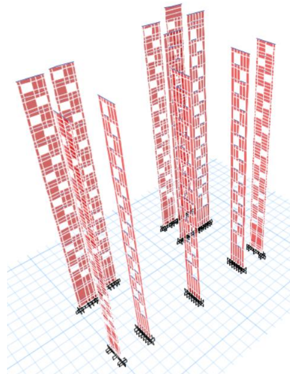
Figure 2: Etabs 3-D View for Staggered Opening (Model-2)
