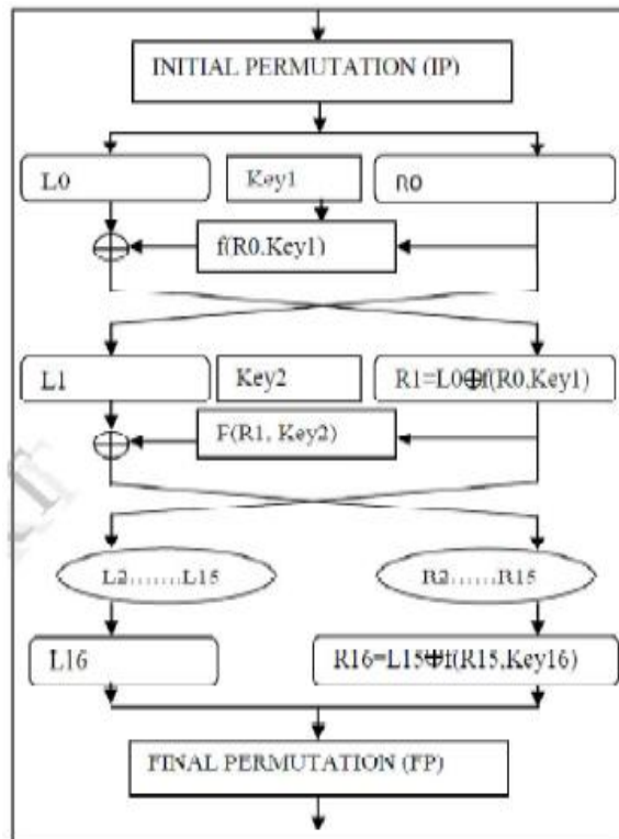
Figure 1: DES algorithm
