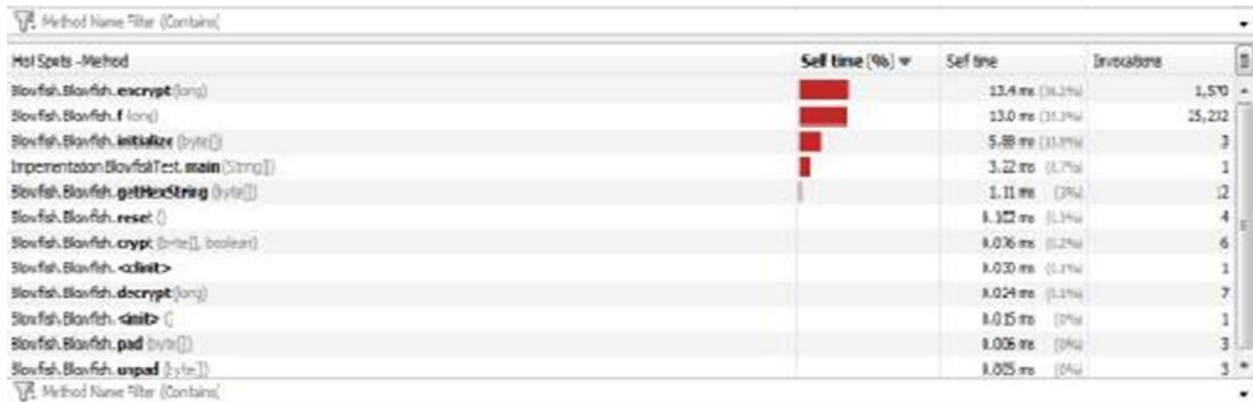
Figure13Encryptiontimeofstandardalgorithm&amp;modified algorithm
