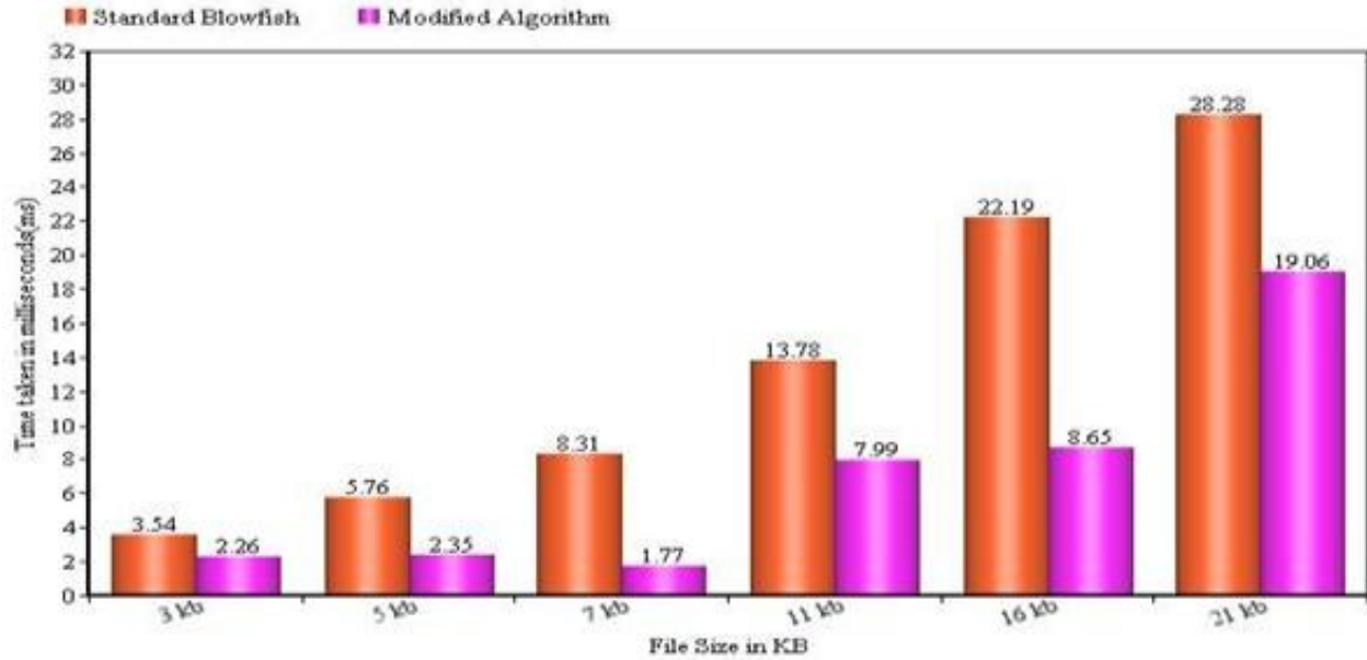
Graph4.1 Comparison of encryption of standard blowfish & modified implementation
