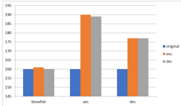
Figure 9 Comparison of AES, DES and Blowfish algorithm
