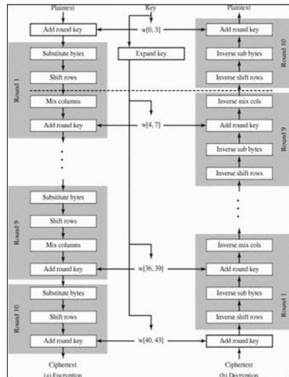
Figure 2: AES algorithm
