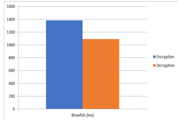
Figure 10 Encryption Decryption Graph for Improved Blowfish Algorithm
