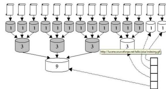
Figure 6: Working of Lucene indexing
