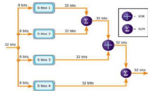
Figure 8 Modified Function F(x)
