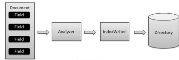
Figure 5: Indexing Process
