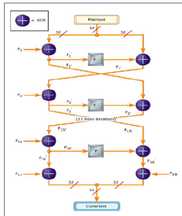
Fig 7: Blowfish Algorithm
