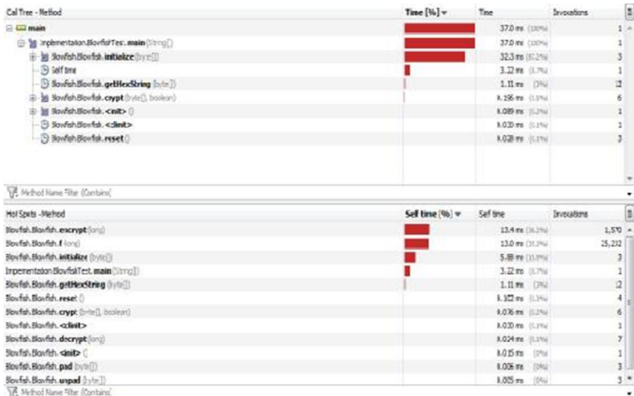
Figure4.2Encryptiontimeofstandardalgorithm&amp;modified algorithm
