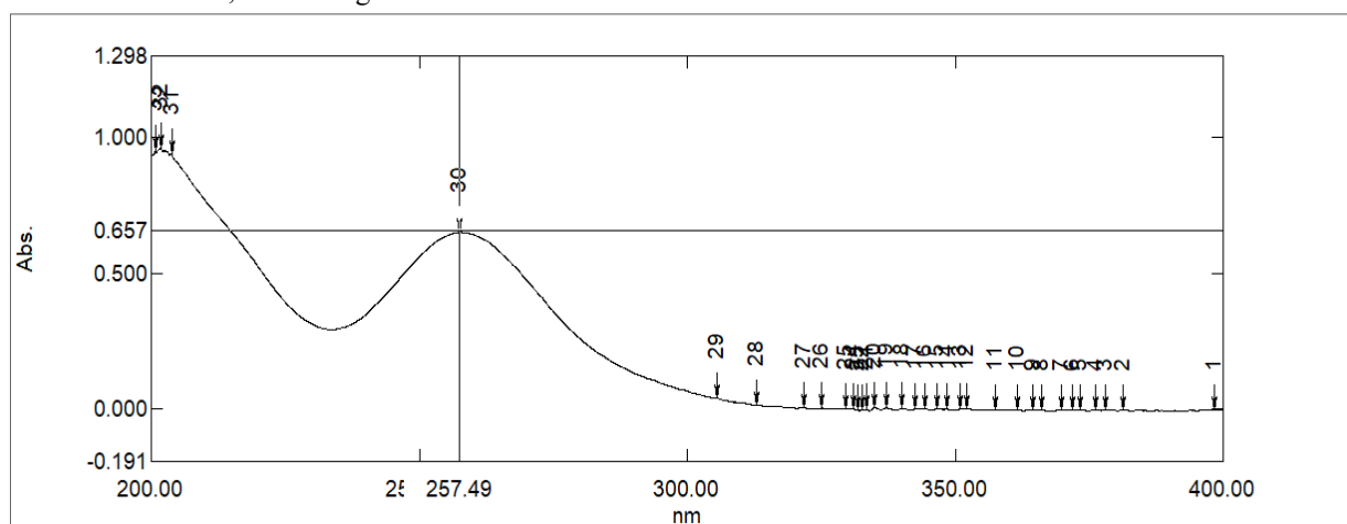
Fig. 2: Overlay spectrum of ketoprofen from the UV-Visible spectrophotometric identification test
