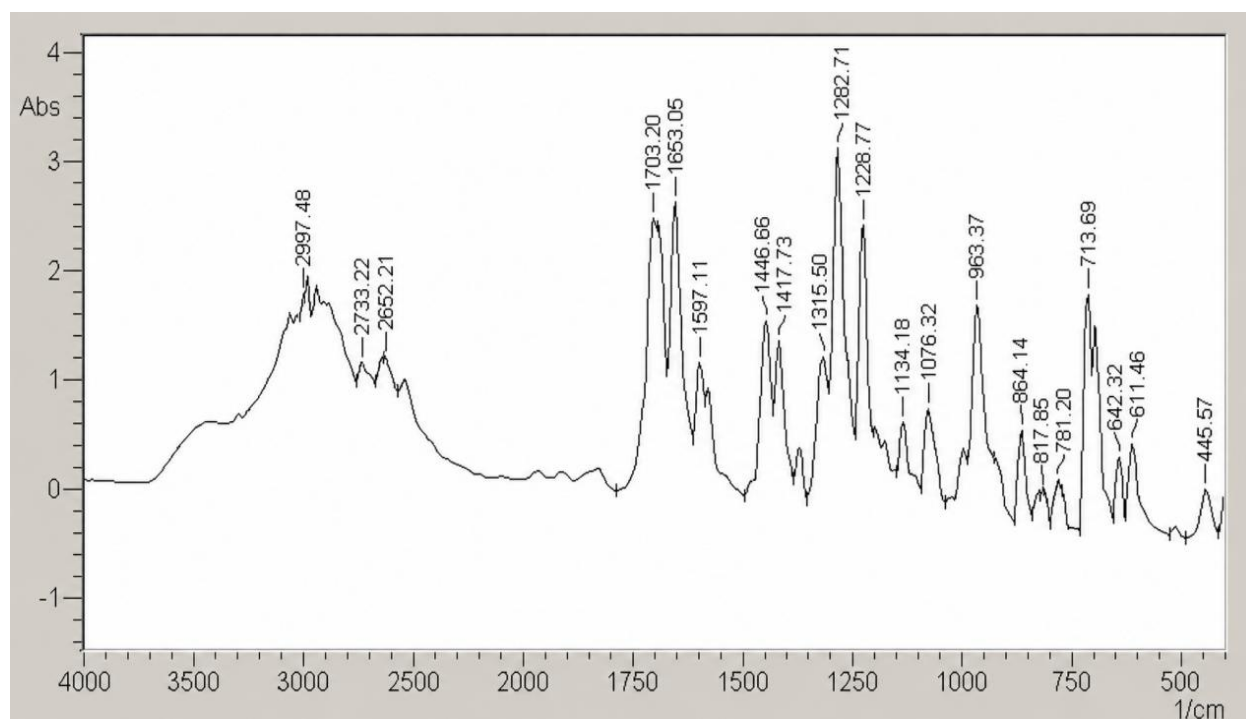
Fig. 3: FTIR spectrum of pure ketoprofen showing characteristic absorption peaks corresponding to its functional groups.
