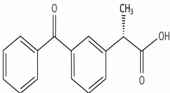
Fig. 1: Chemical structure of Ketoprofen
