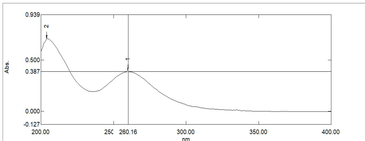
Fig. 4: UV-Visible absorption spectrum of ketoprofen showing maximum absorption
