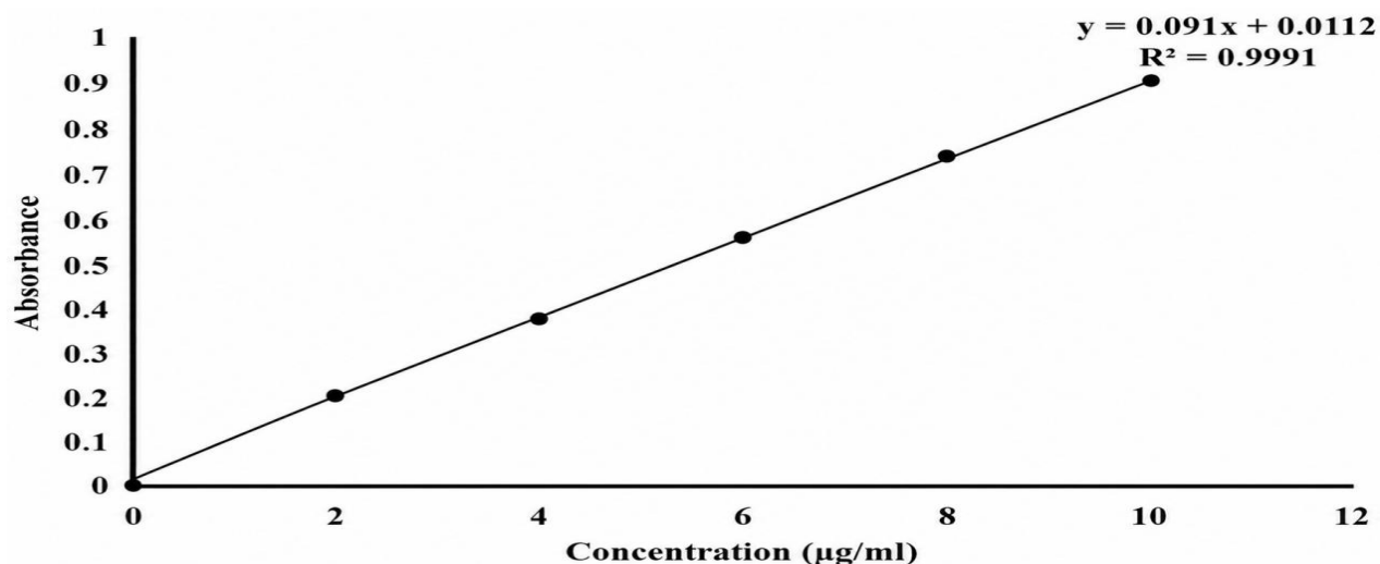
Fig. 5: Calibration curve of ketoprofen in the concentration range of 2–10 µg/mL at 260 nm
