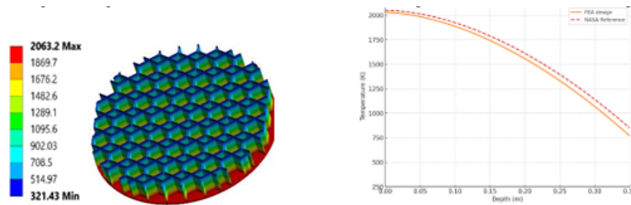
Figure 2: ANSYS simulation of hexagonal honeycomb heat shield and validation with NASA reference data
