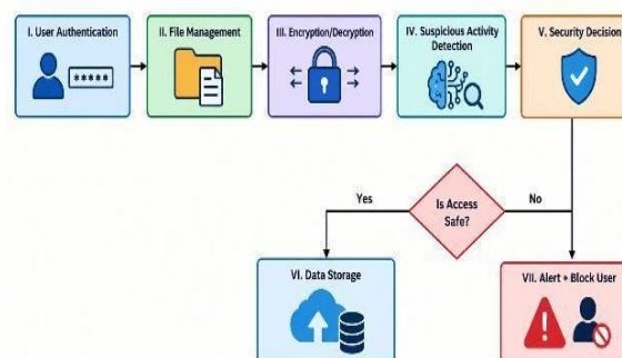
Fig. 4. Proposed system architecture.
