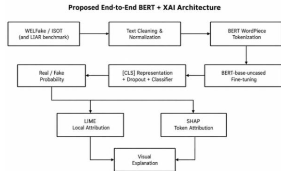
Fig. 1. Proposed end-to-end BERT + XAI system architecture.
