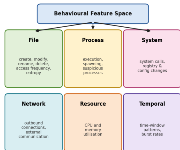
Fig. 3. Behavioural feature categories.
