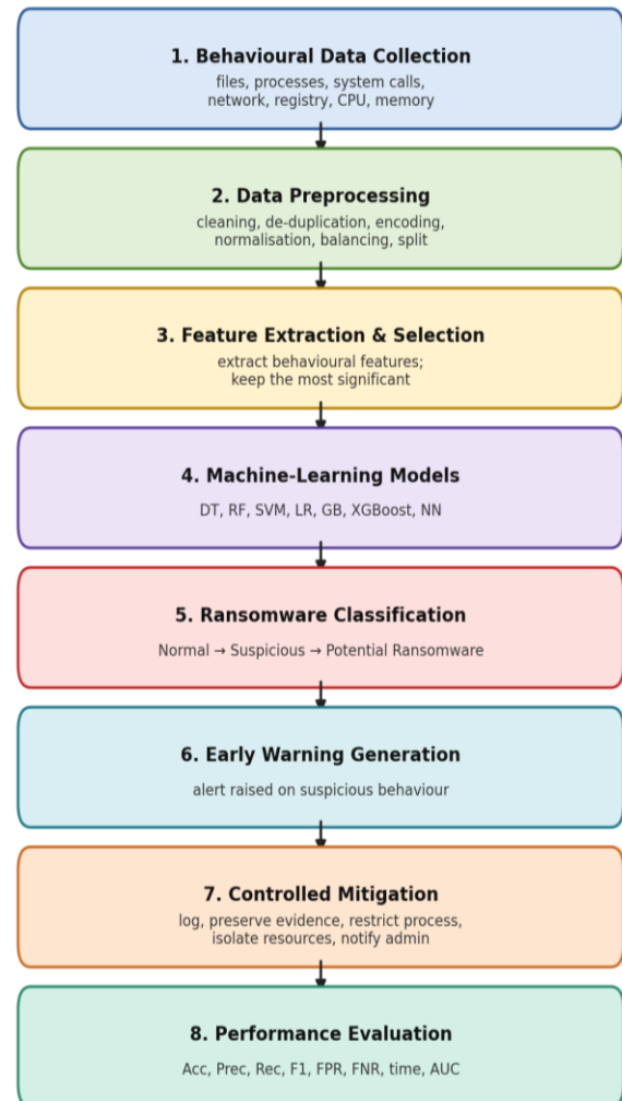
Fig. 4. Proposed framework for early ransomware detection and mitigation
