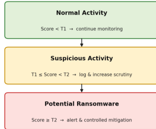
Fig. 2. Ransomware activity classification process.
